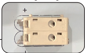
Wago Plug
